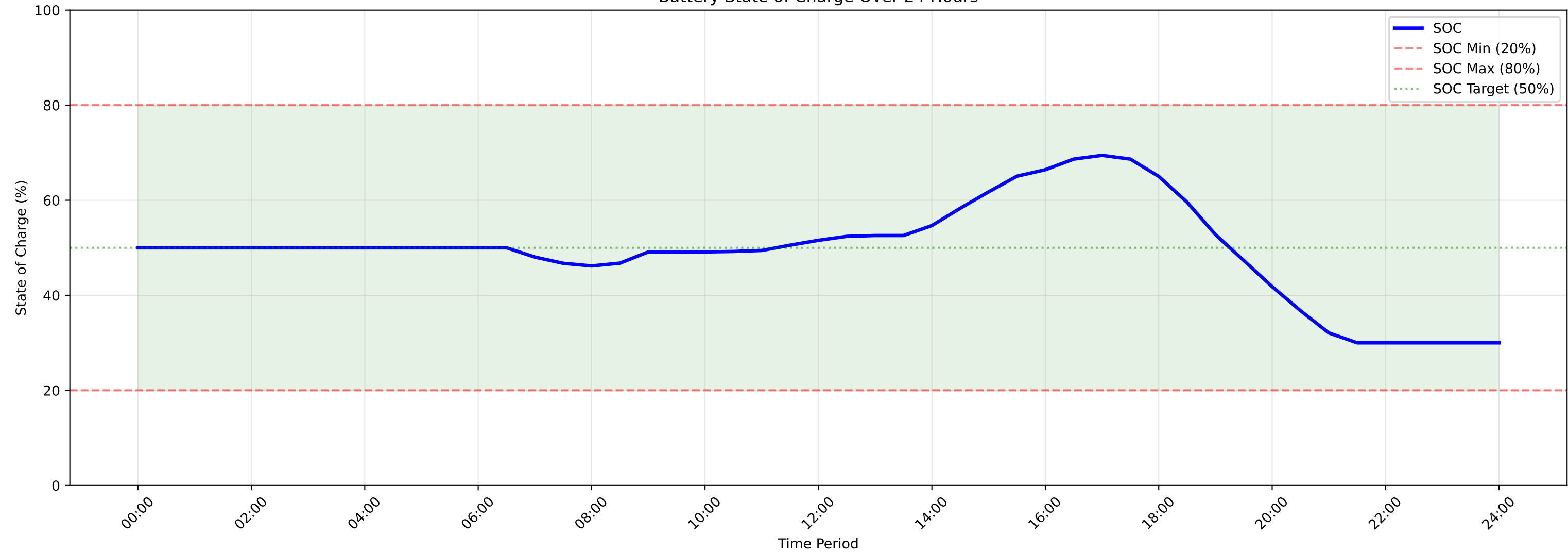
Battery State of Charge Over 24 Hours
